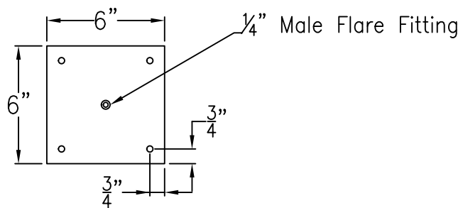
Ceiling Mount
