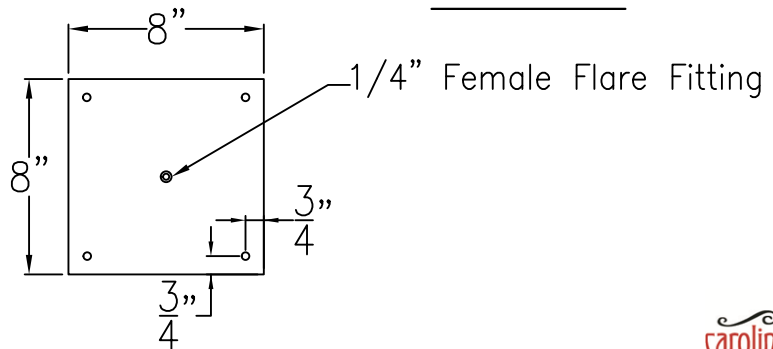
Ceiling Mount
