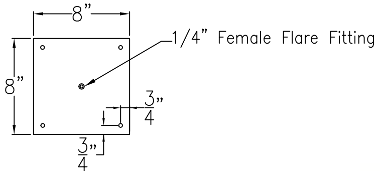
Ceiling Mount
