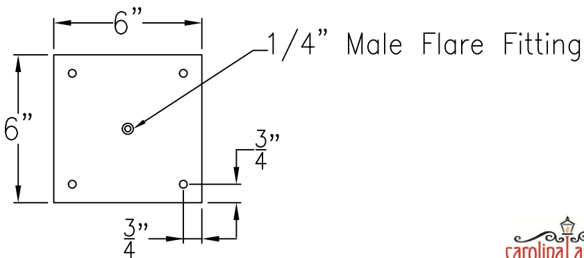
Ceiling Mount
