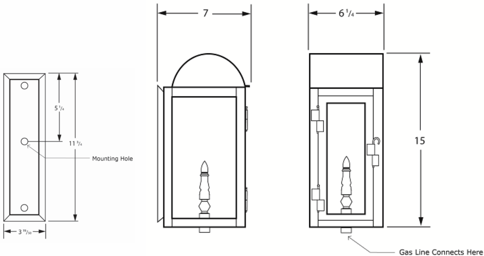
SIDE VIEW
