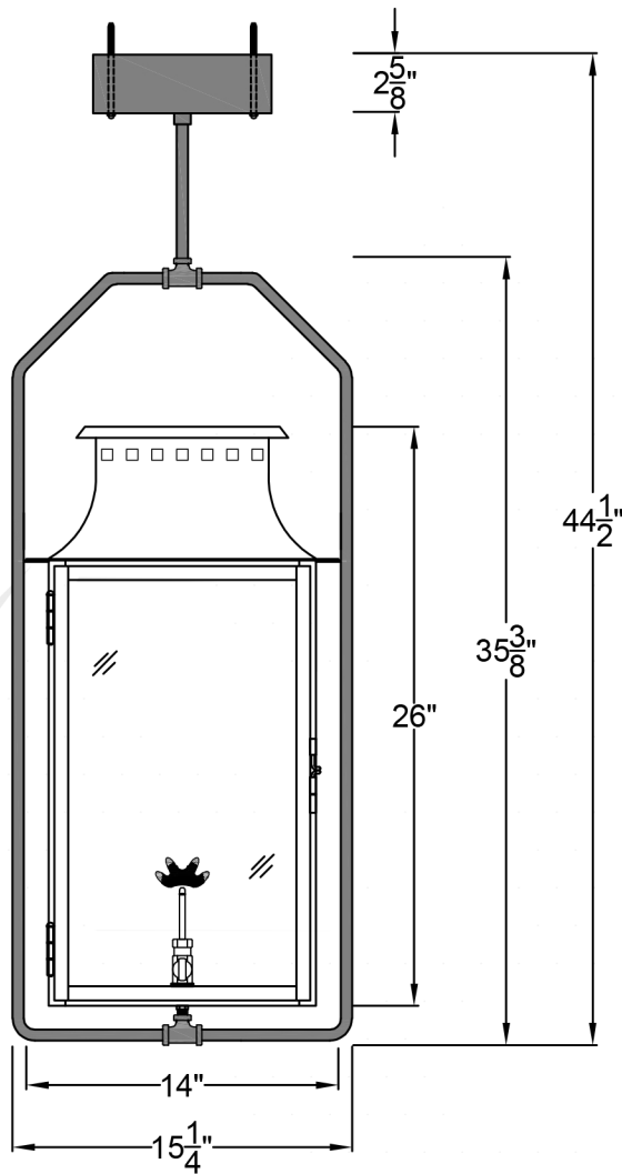
Front View
