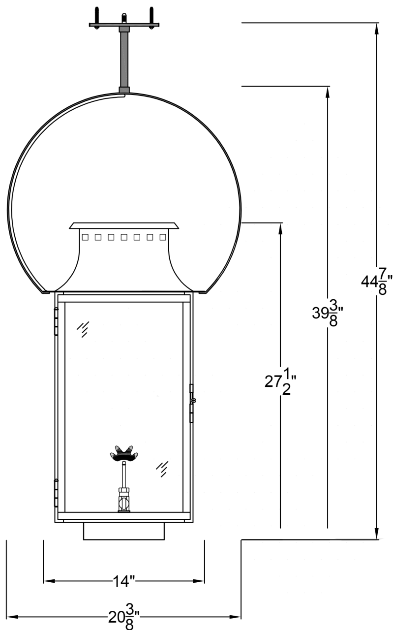
Front View
