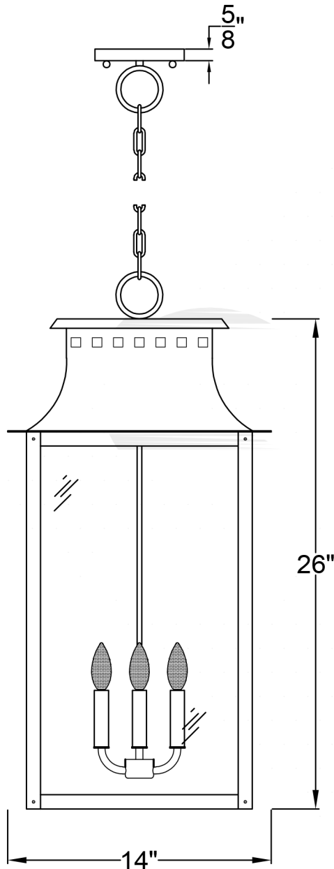
Front View
