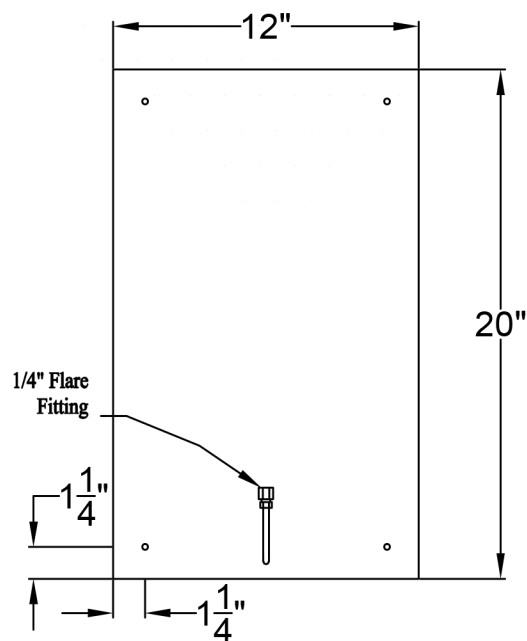
Backplate
