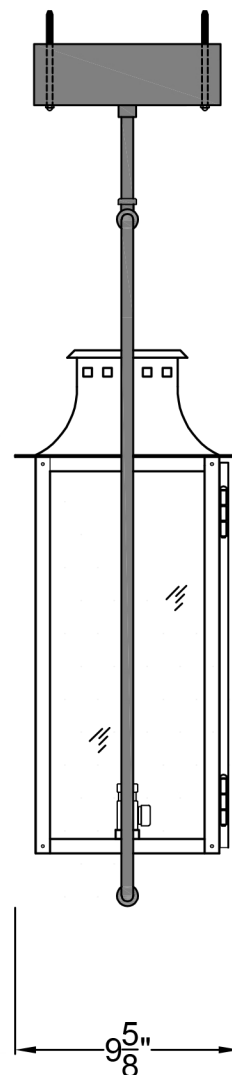
Side View
