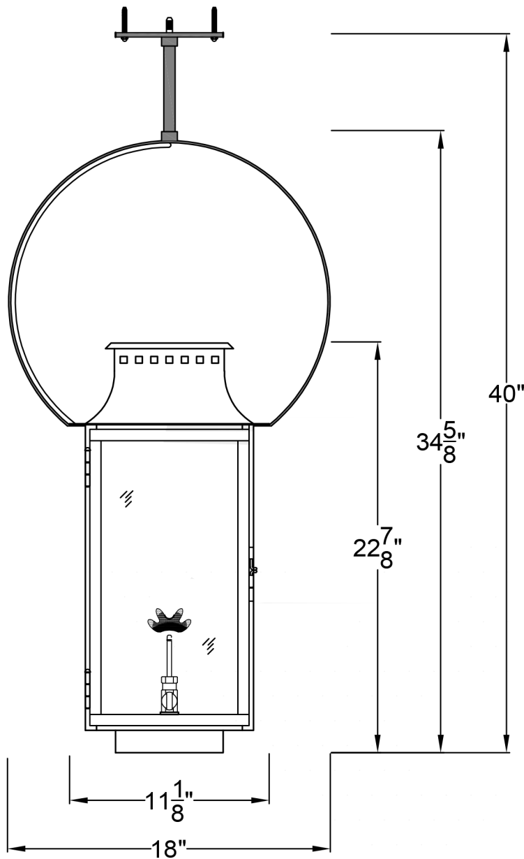
Front View
