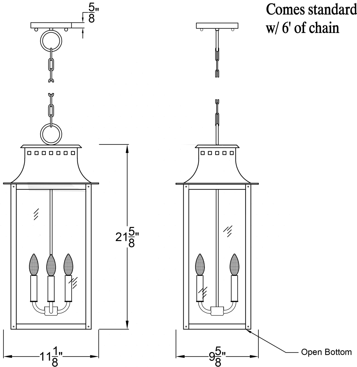
Front View
