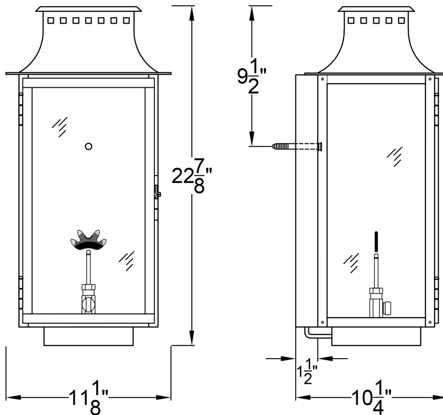
Side View
