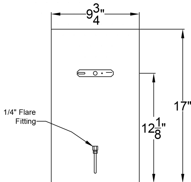
Backplate
