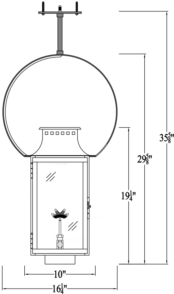
Front View
