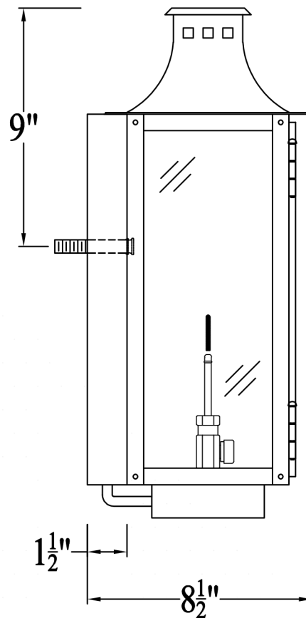
Side View
