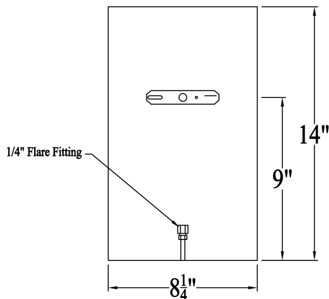
Backplate
