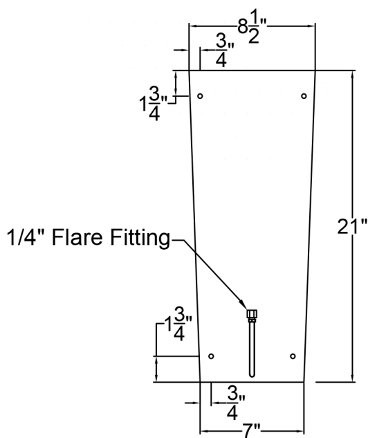
Backplate
