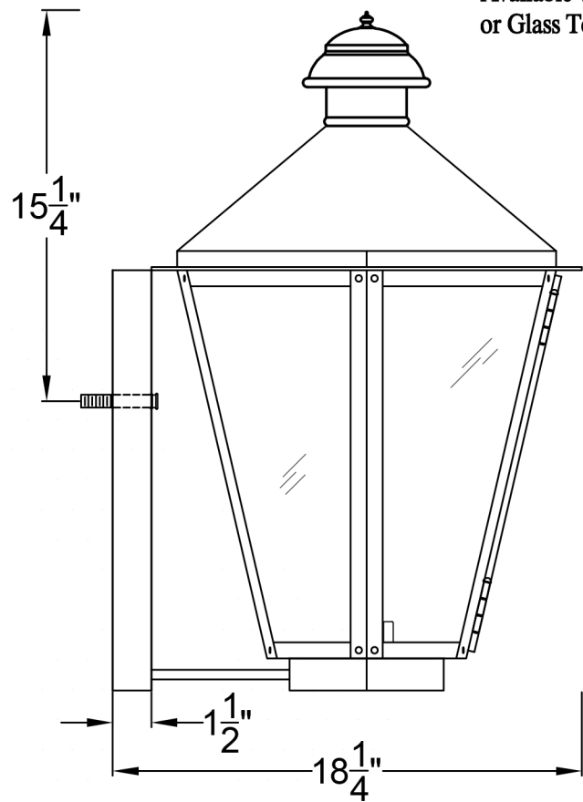
Side View
