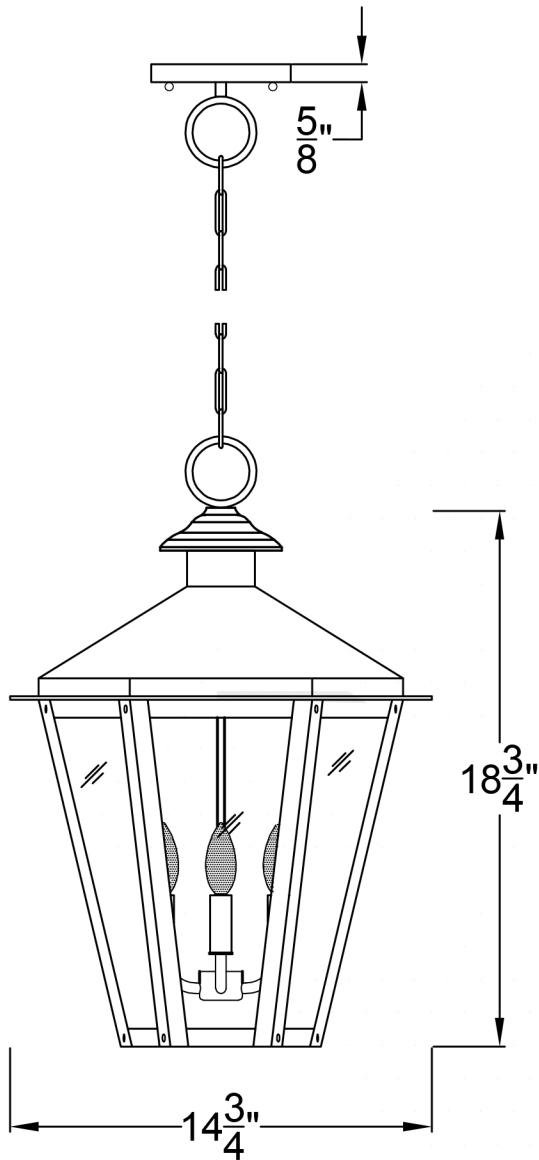
Front View
