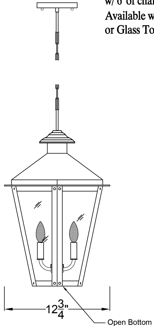
Side View
