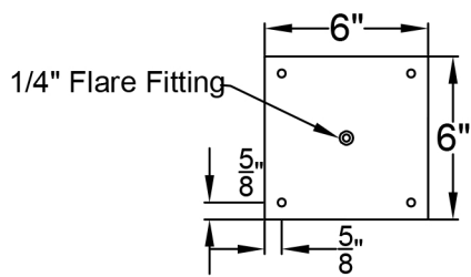
Ceiling Mount
