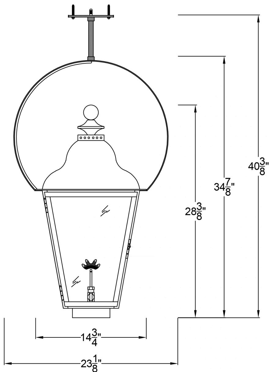
Front View
