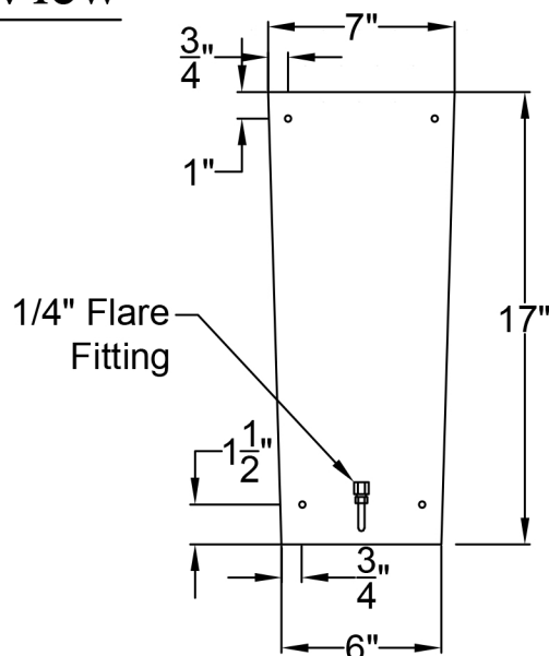
Backplate
