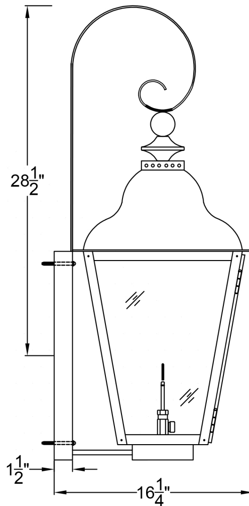
Side View
