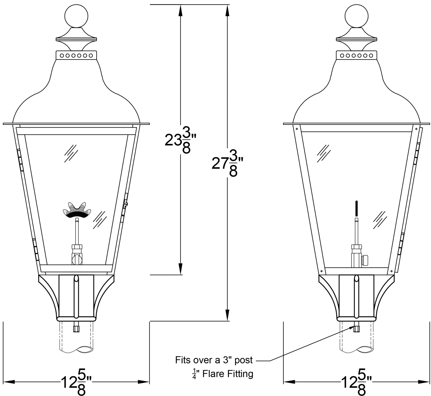
Front View
