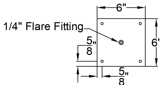
Ceiling Mount
