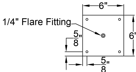
Ceiling Mount
