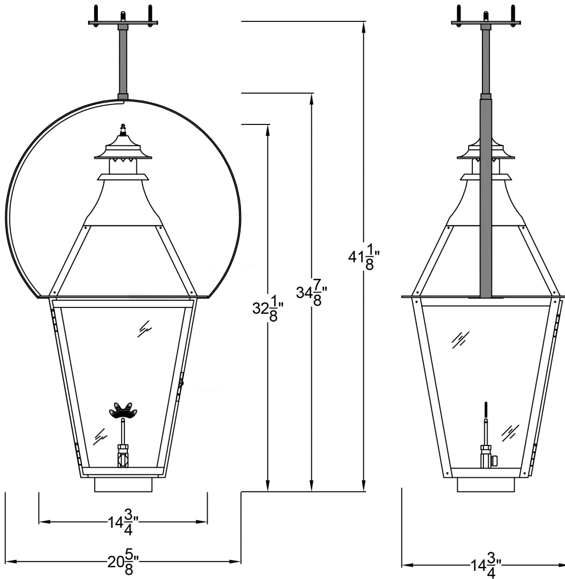
Side View
