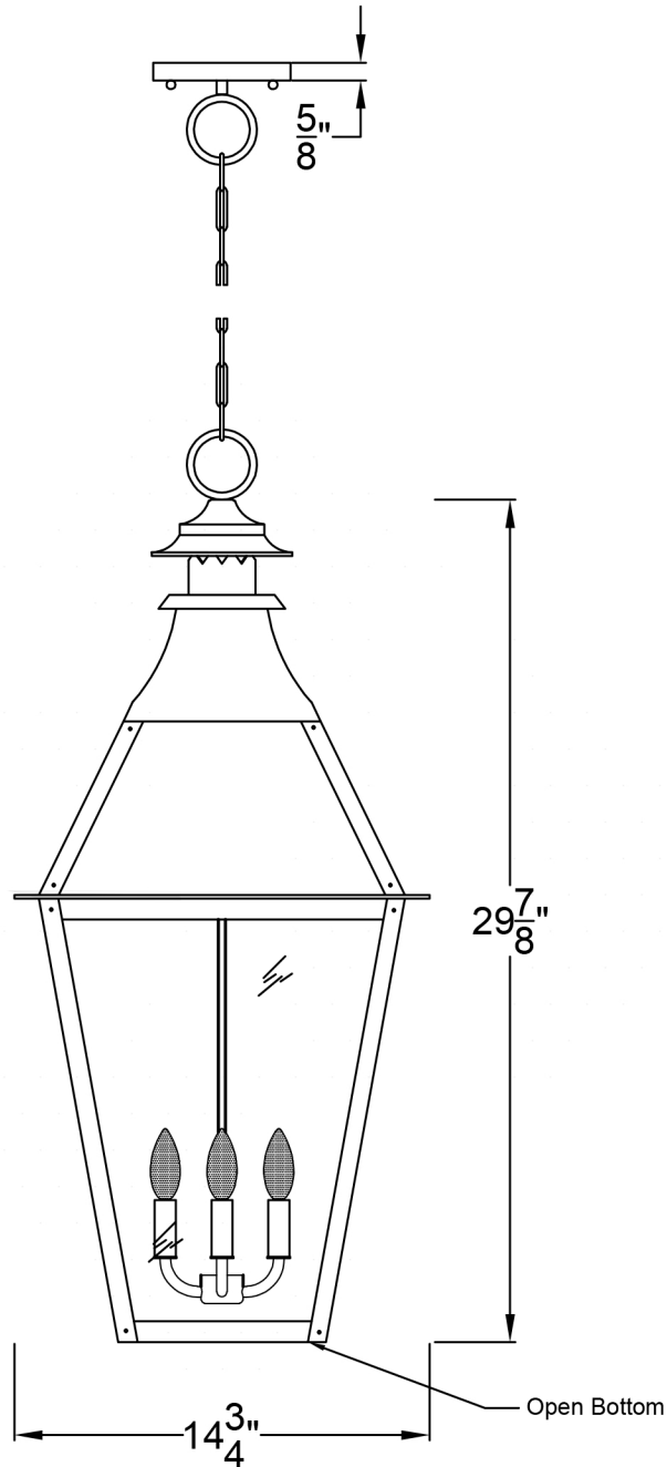
Front View
