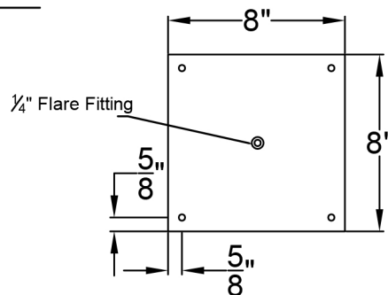
Ceiling Mount
