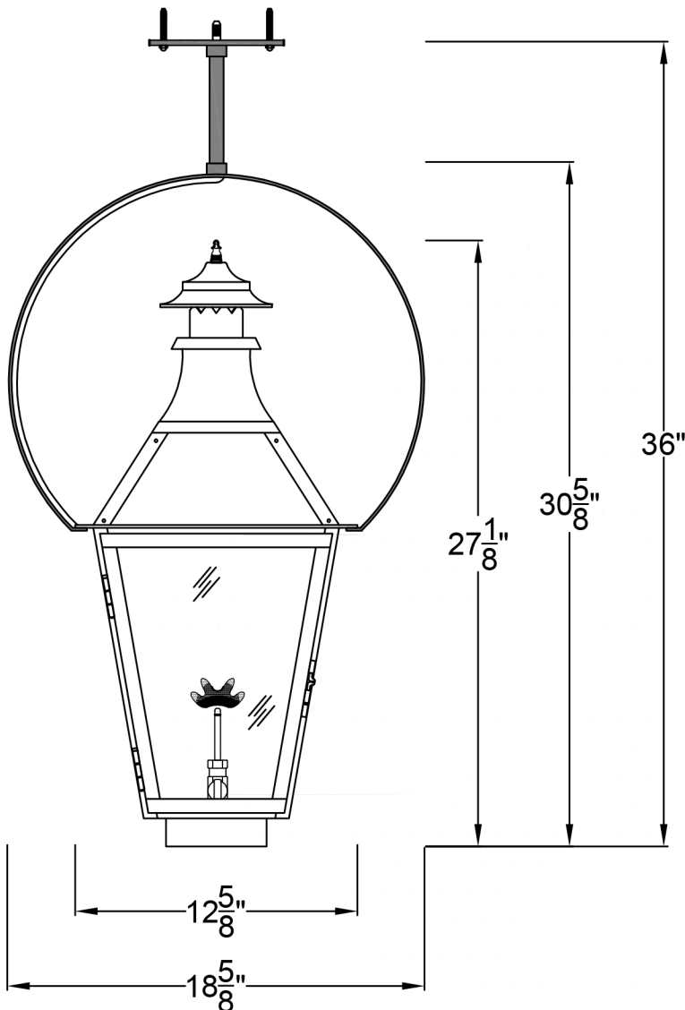
Front View
