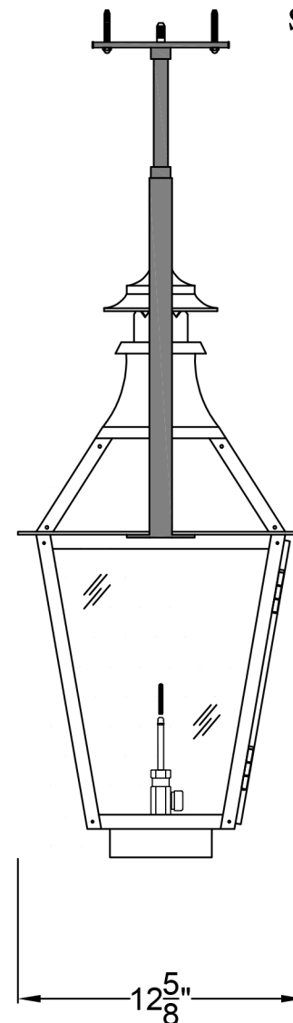
Side View
