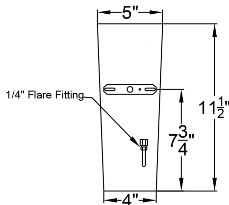
Backplate
