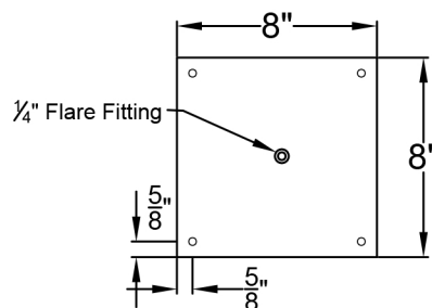
Ceiling Mount
