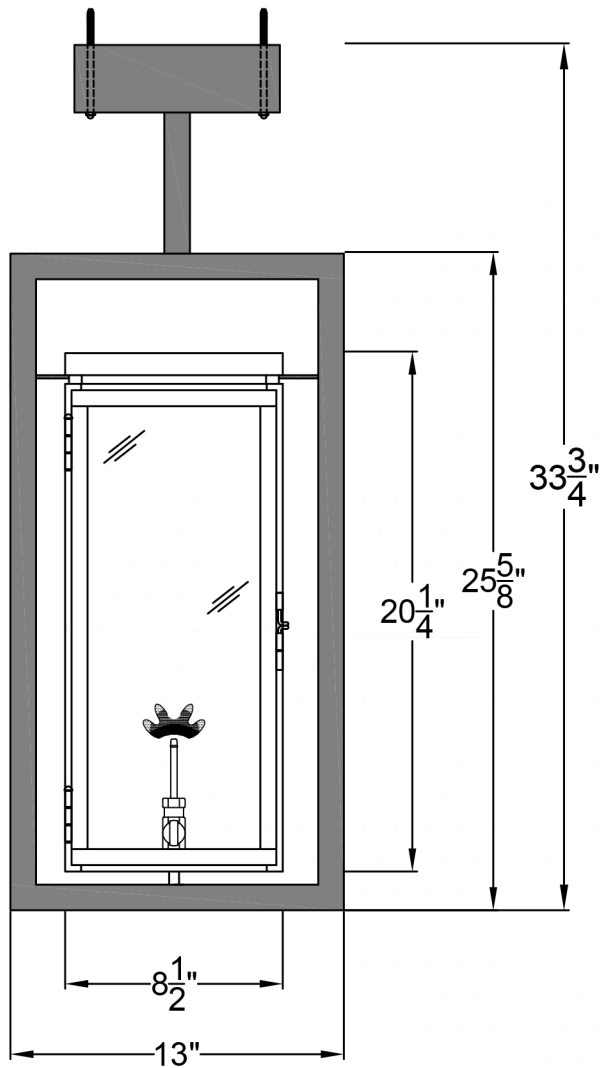
Front View
