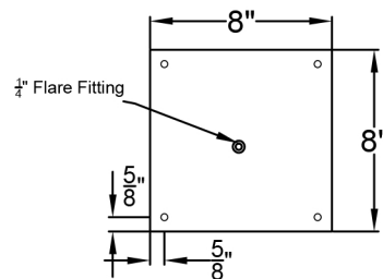
Ceiling Mount
