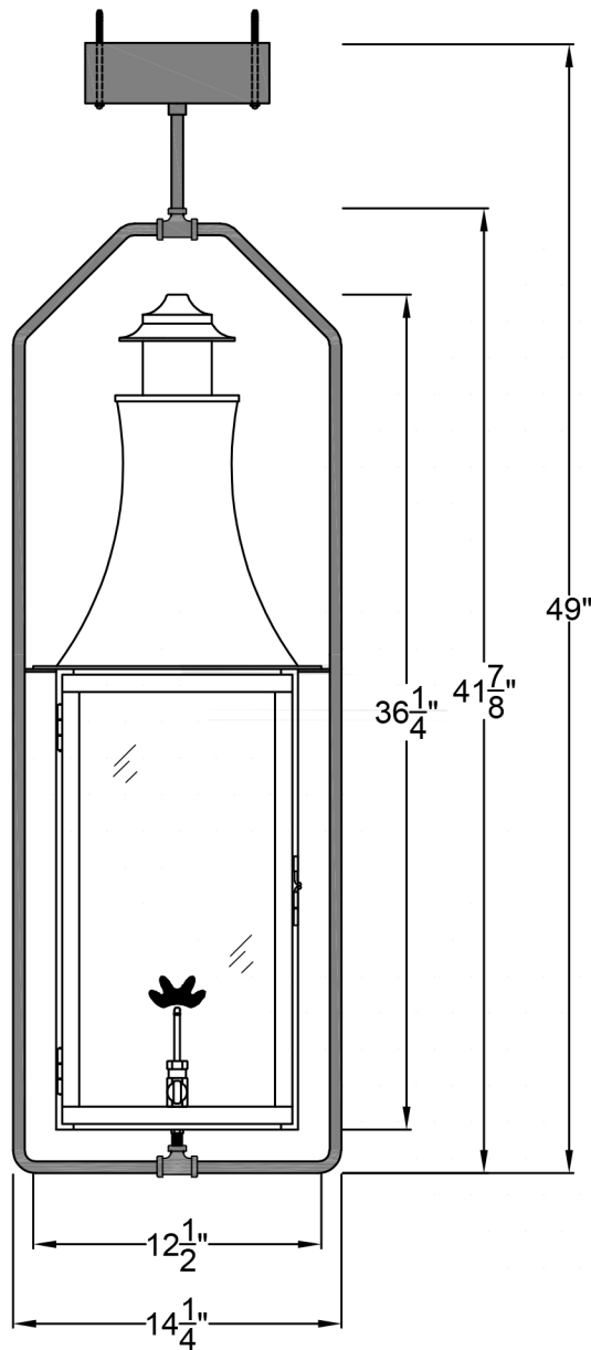
Front View
