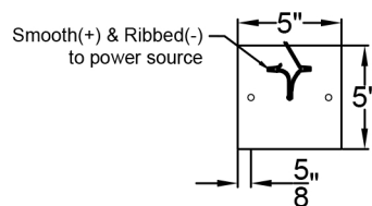
Ceiling Canopy
