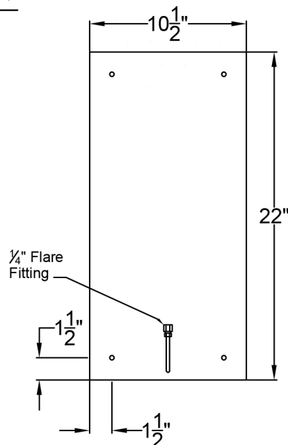
Backplate
