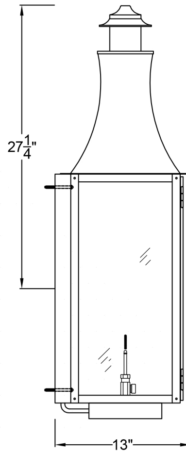
Side View
