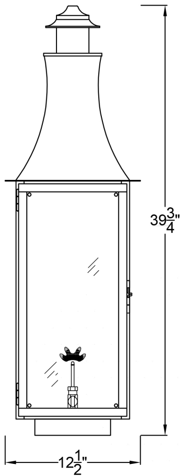
Front View
