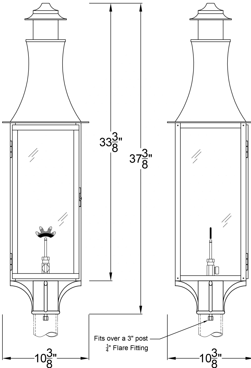
Front View
