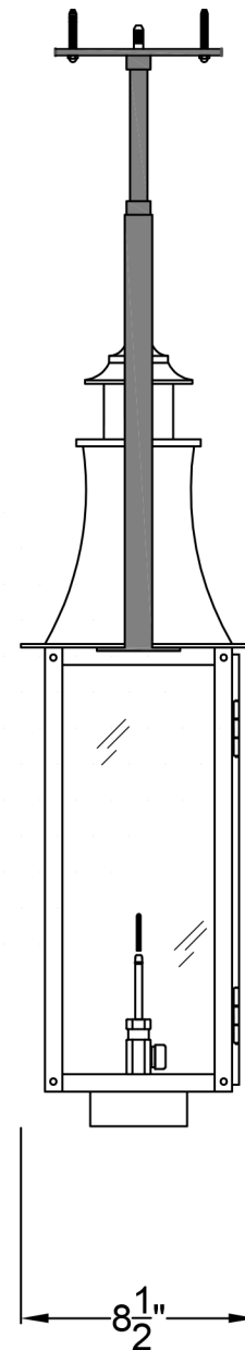
Side View
