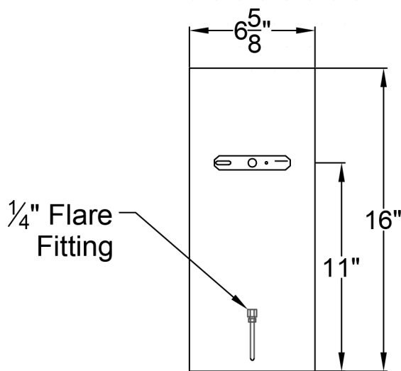
Backplate
