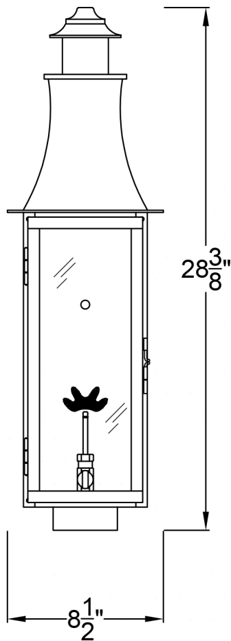
Front View
