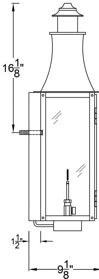
Side View
