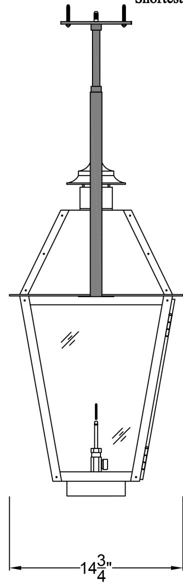
Side View
