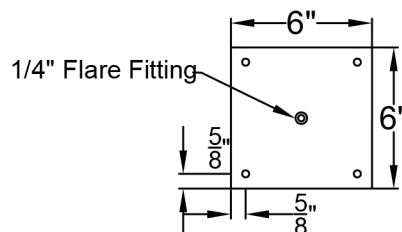
Ceiling Mount
