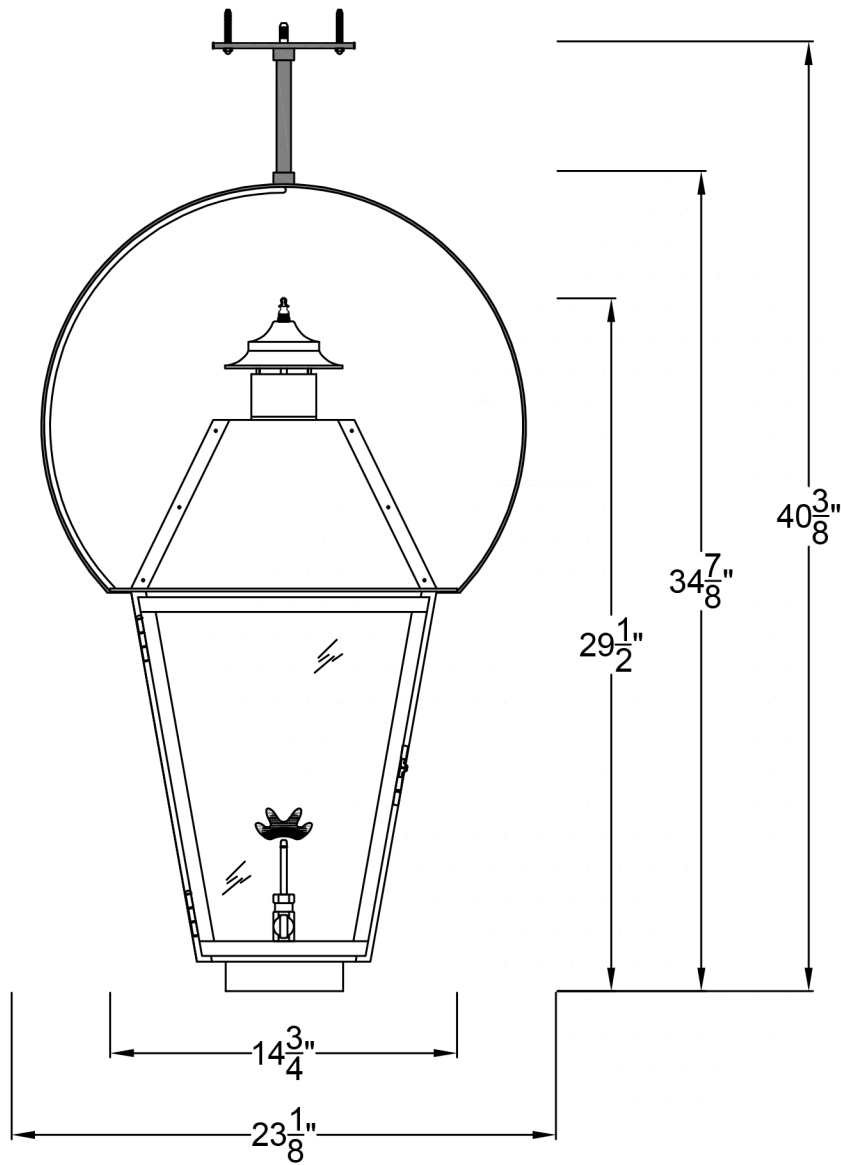
Front View
