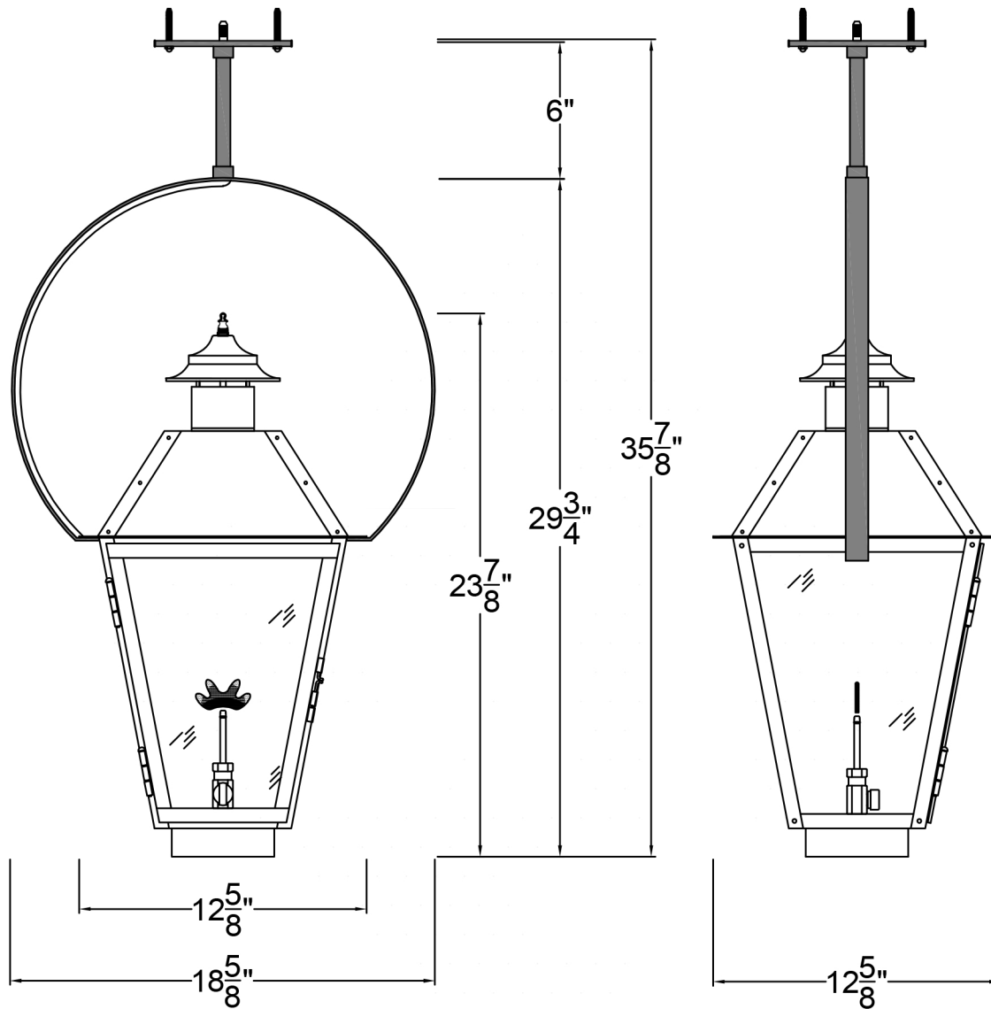
Front View
