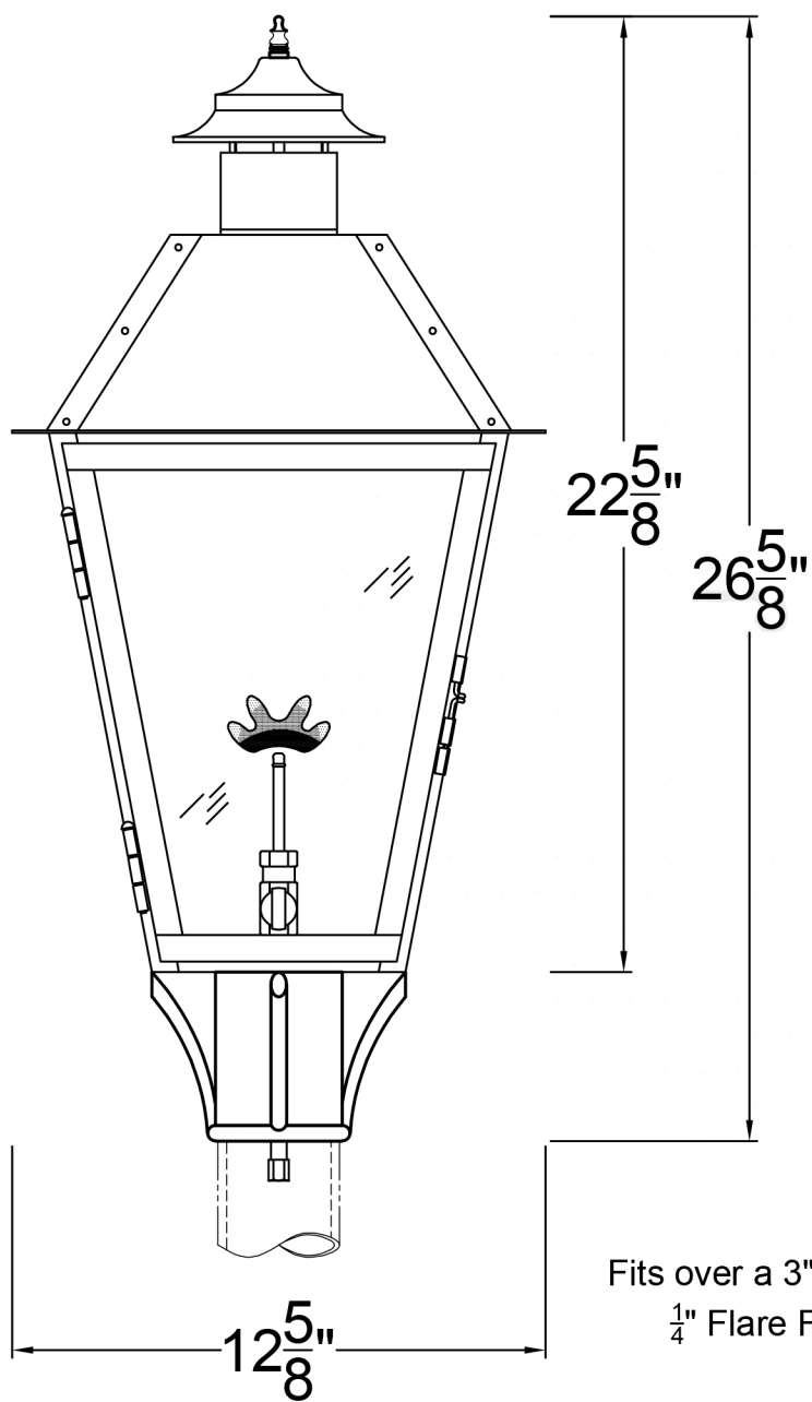
Front View
