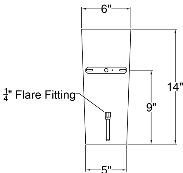
Backplate
