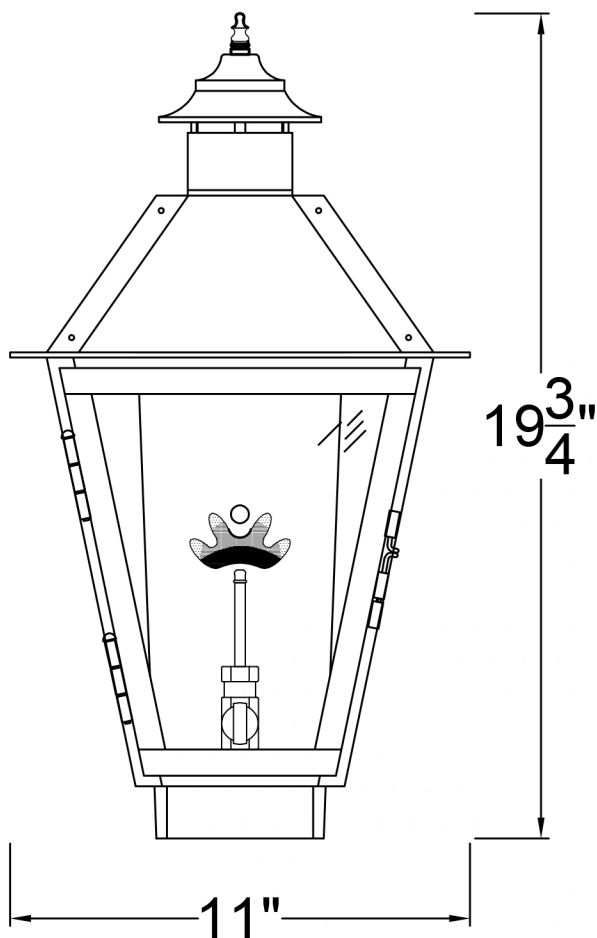
Front View
