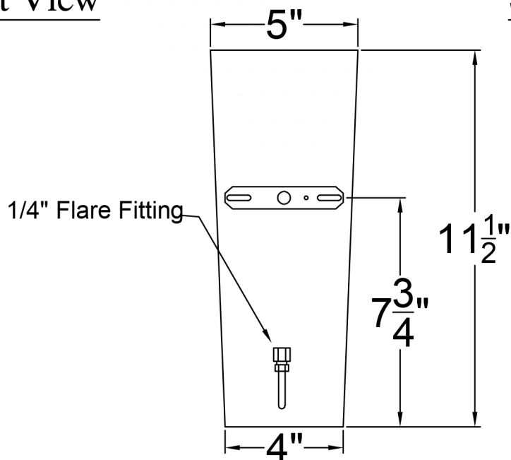
Backplate
