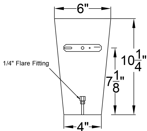
Backplate
