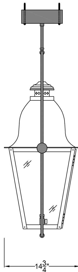
Side View
