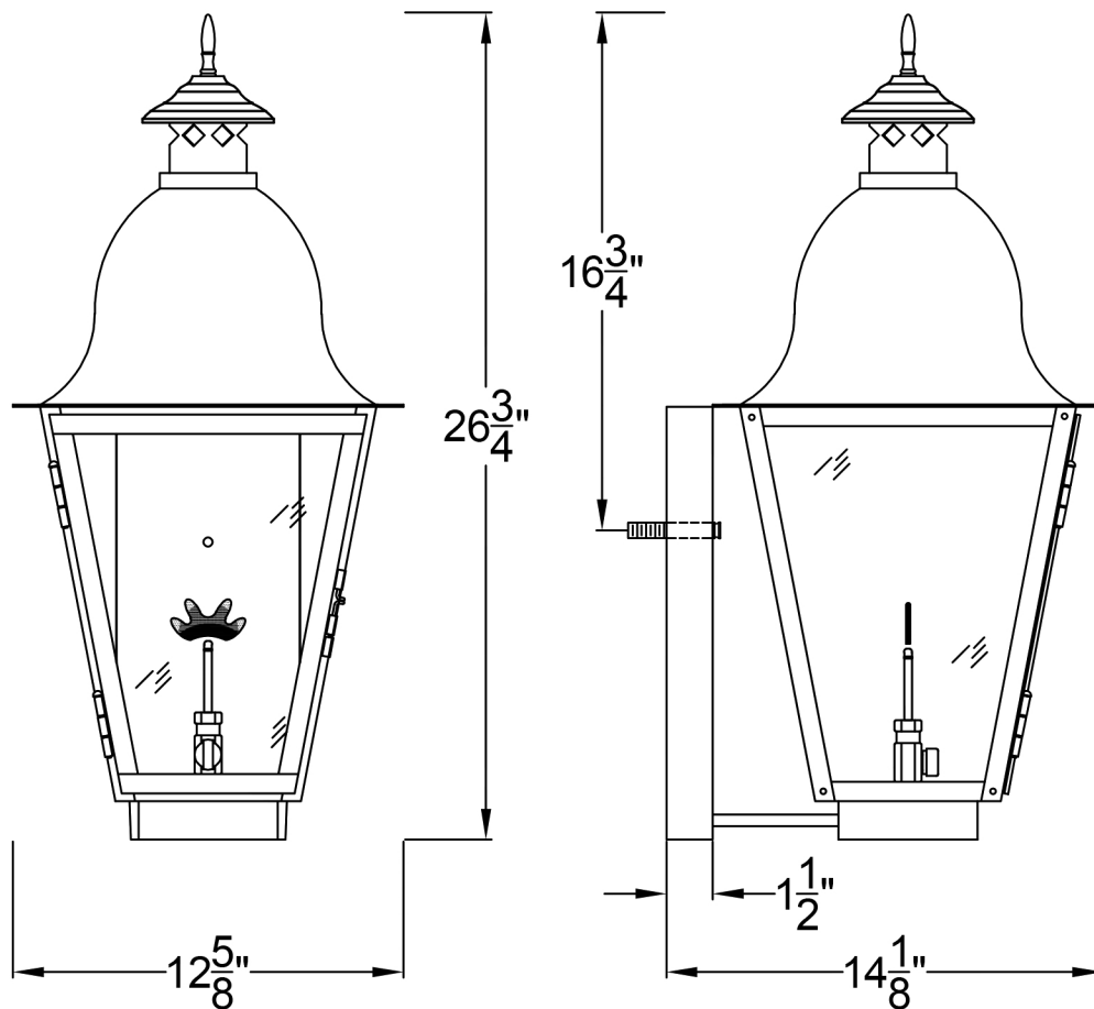
Front View
