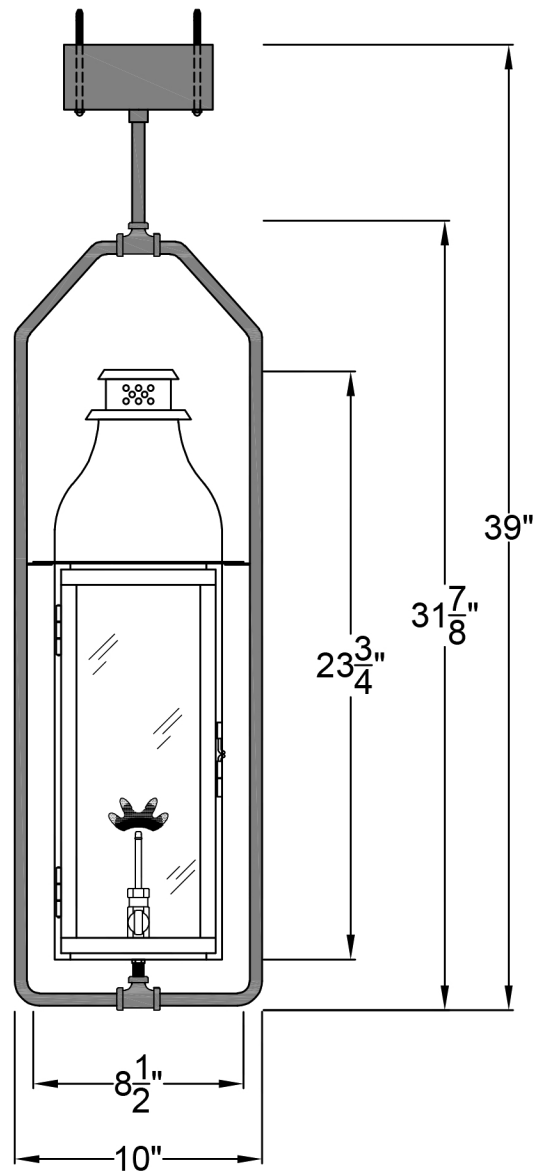
Front View
