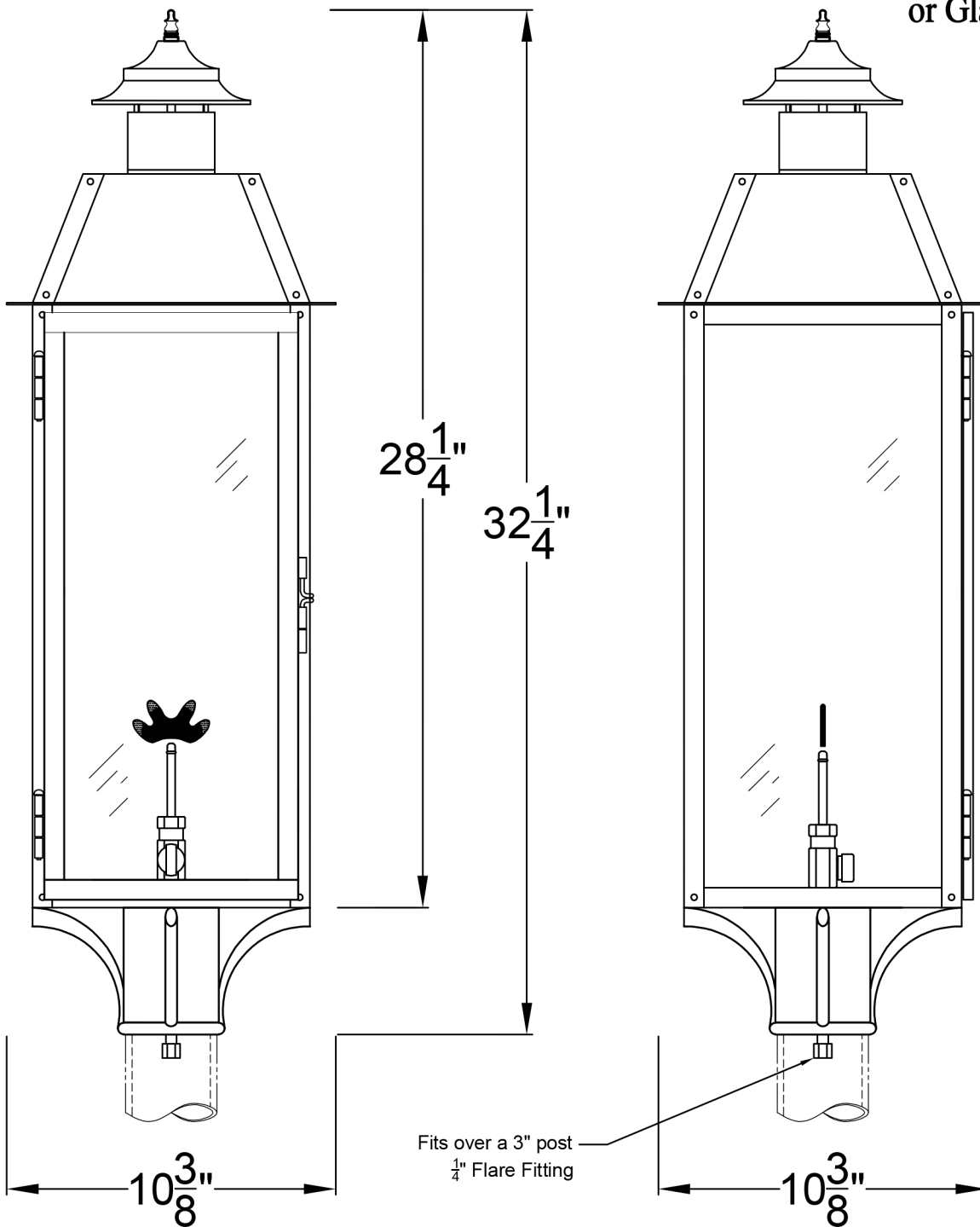
Front View
