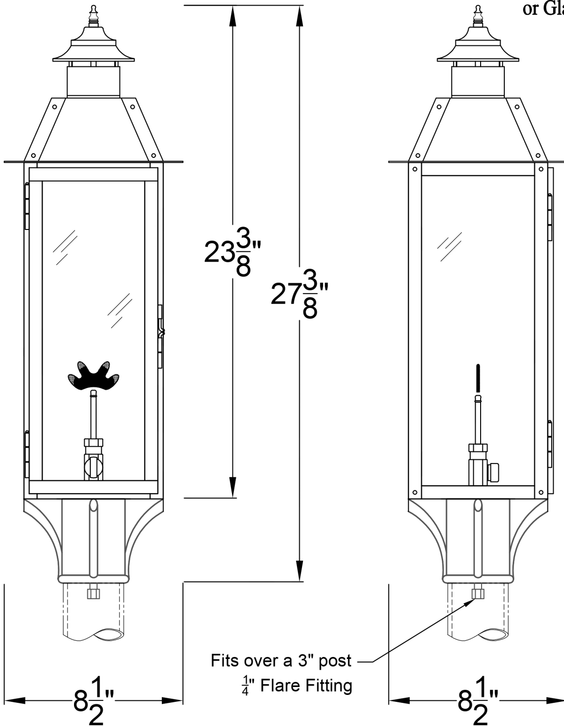
Side View
