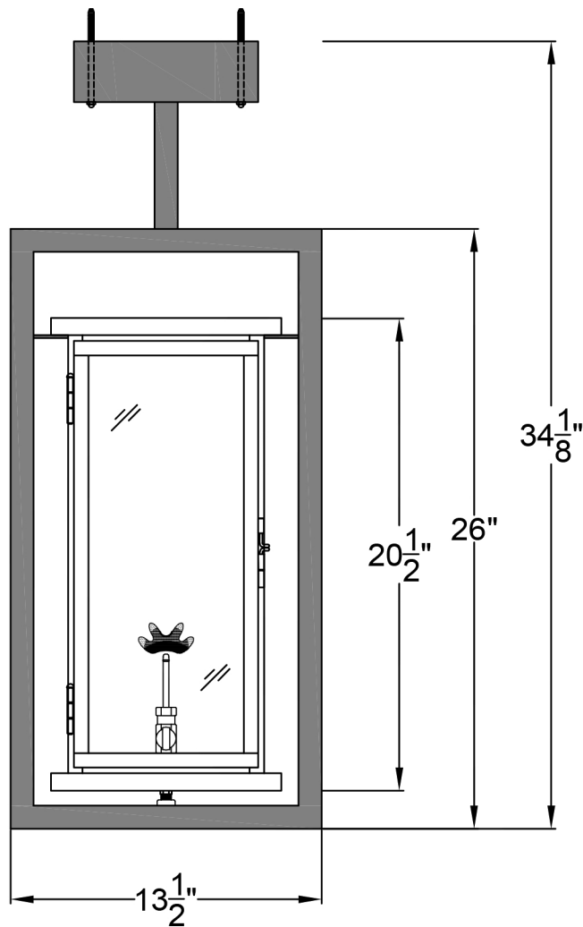
Front View
