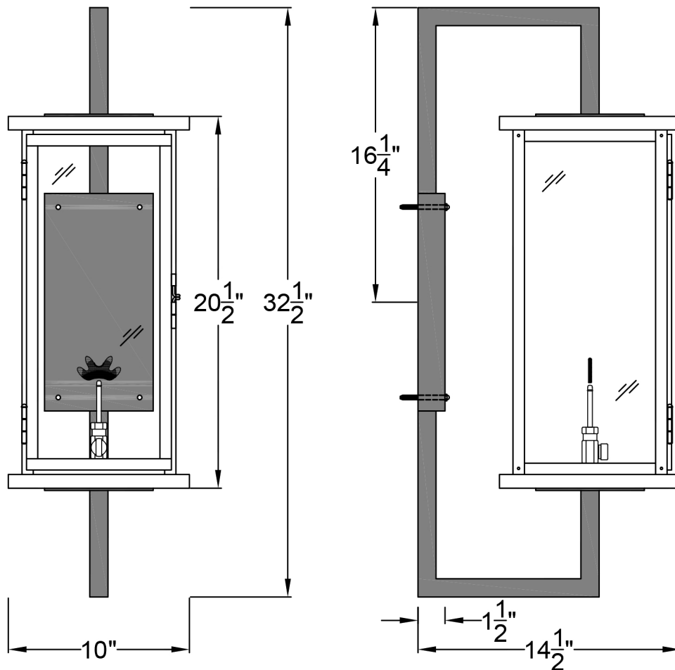
Front View
