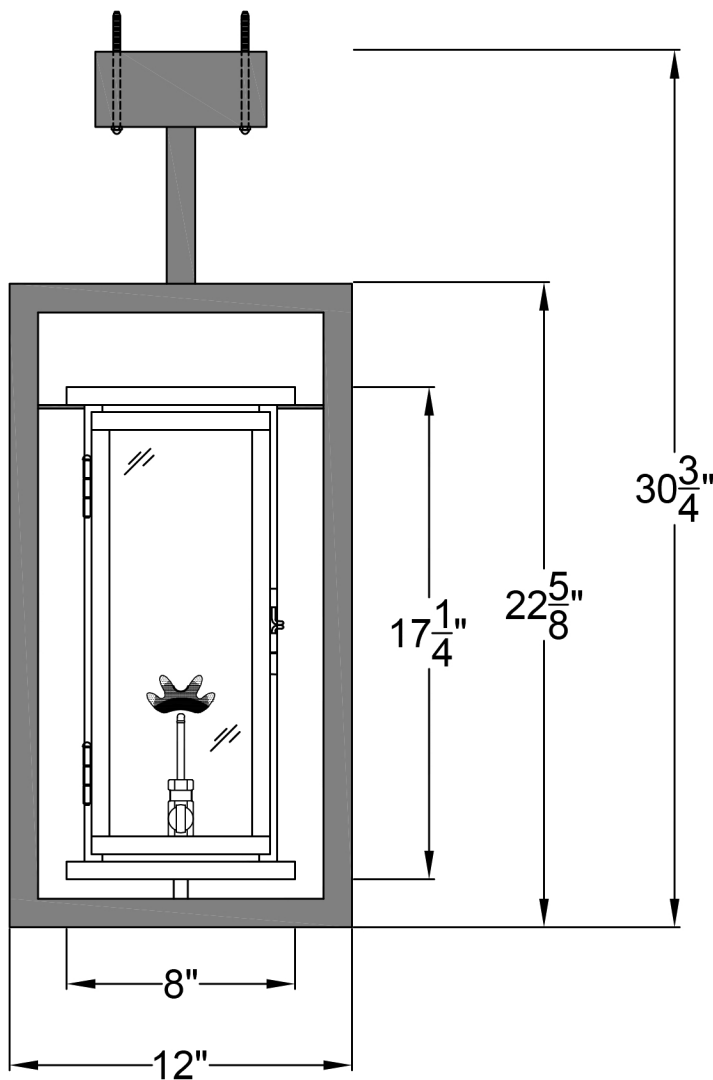
Front View
